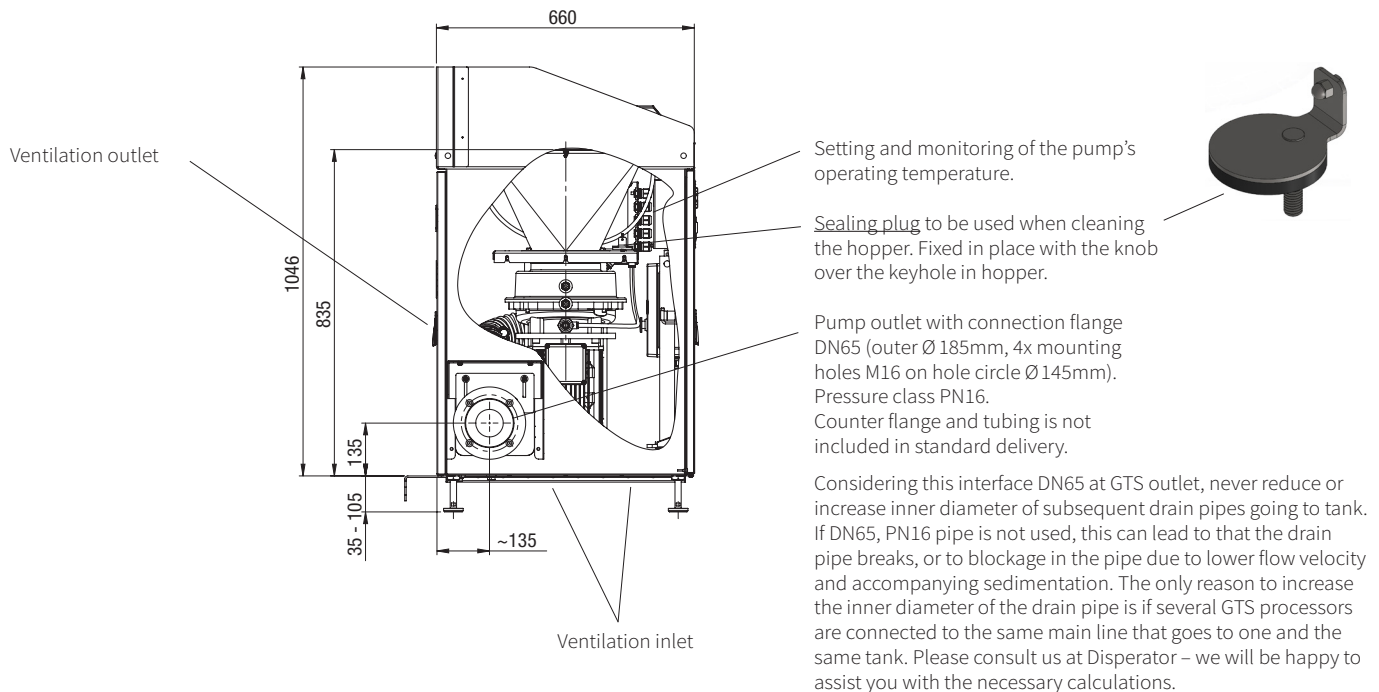
Side view
